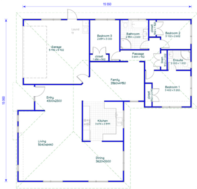
Floor Plan
