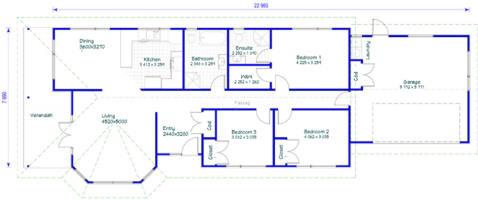
Floor Plan
