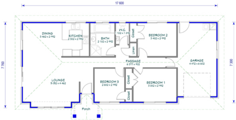
Floor Plan
