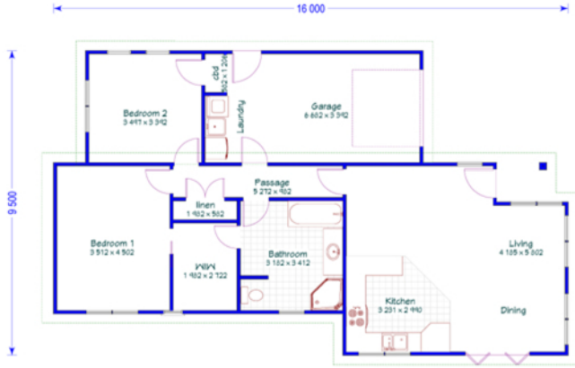
Floor Plan
