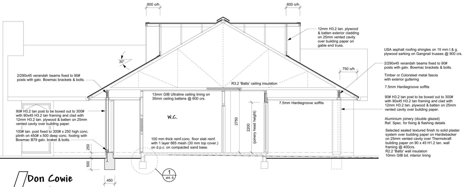
SECTION E-E
